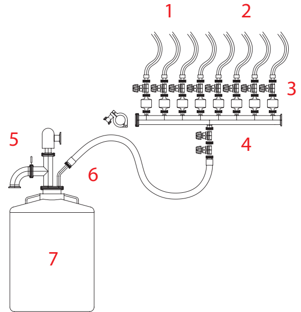
TYPICAL BIOPHARM SYSTEM
