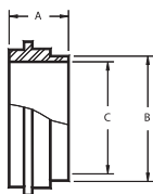
14AJP JOHN PERRY TYPE FERRULE (LONG)
