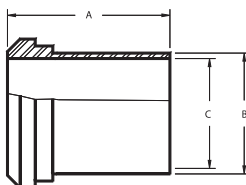
14W PLAIN FERRULE TANK SPUD (HEAVY)
