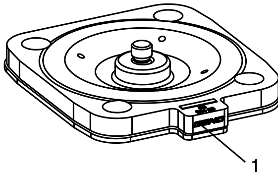
Fig. 1: Diaphragm RFID chip
